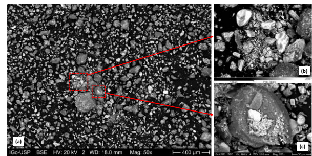
Fig. 3 Photomicrographs on a 400 \mu\text{m} scale with grains ranging from sub-rounded to angular, consisting predominantly of quartz grains; (b) and (c) Presence of fine to powdery material adhered to the quartz grains.
