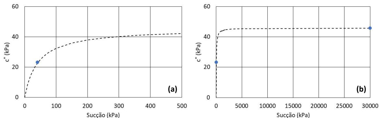
Fig 7. Shear strength envelope obtained (a) for low suction values and added experimental data (b) complete envelope.
